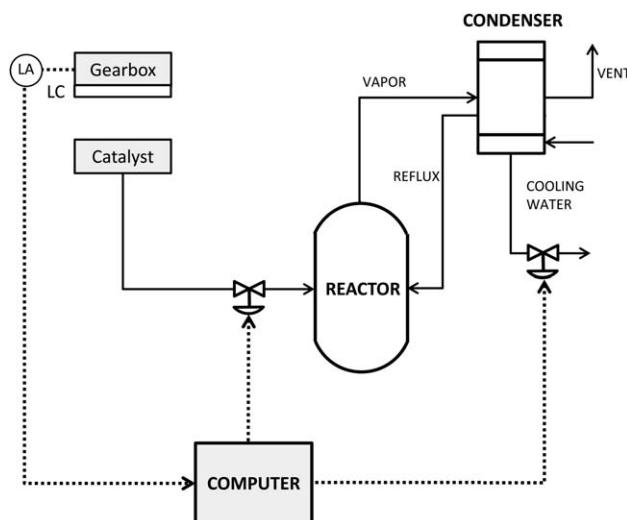
Figure 2. Batch reactor system (adapted from Kletz, 1982).
