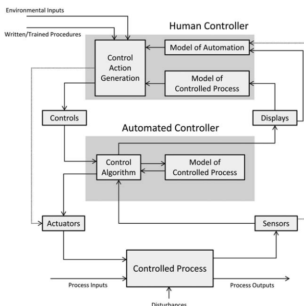
Figure 5. A typical control loop and the associated model-predictive controllers to ensure the satisfaction of the safety constraints.
