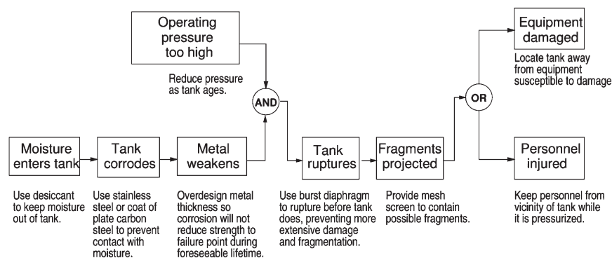
Figure 1. An example chain-of-events model for a tank rupture (Leveson, 2012).
